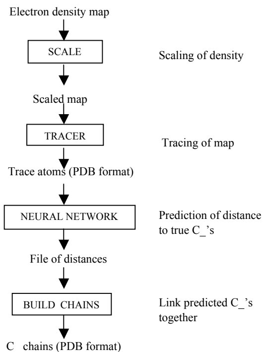
Fig. 3. Steps within CAPRA.
