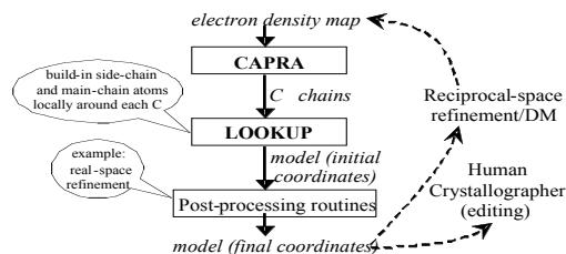
Fig. 2. Main stages of TEXTAL.
