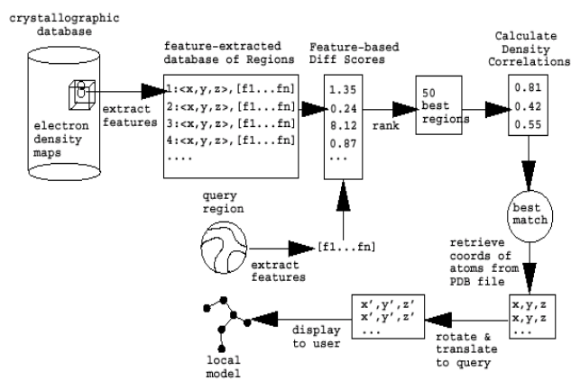
Fig. 4. The LOOKUP process.
